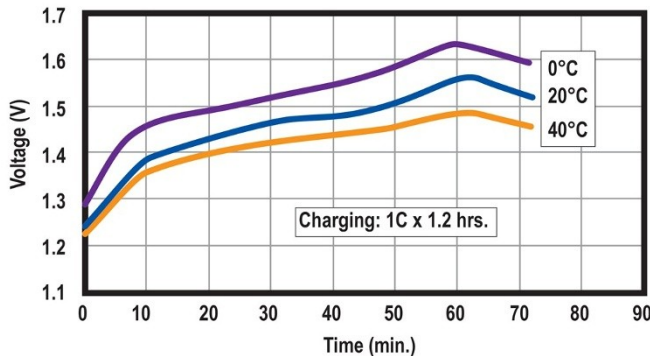
Fast Charge
