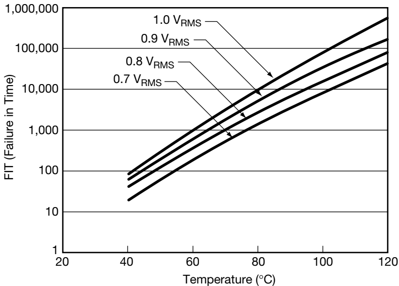
FIT OF VARISTORS ( V_{rms} \leq 40 V )
