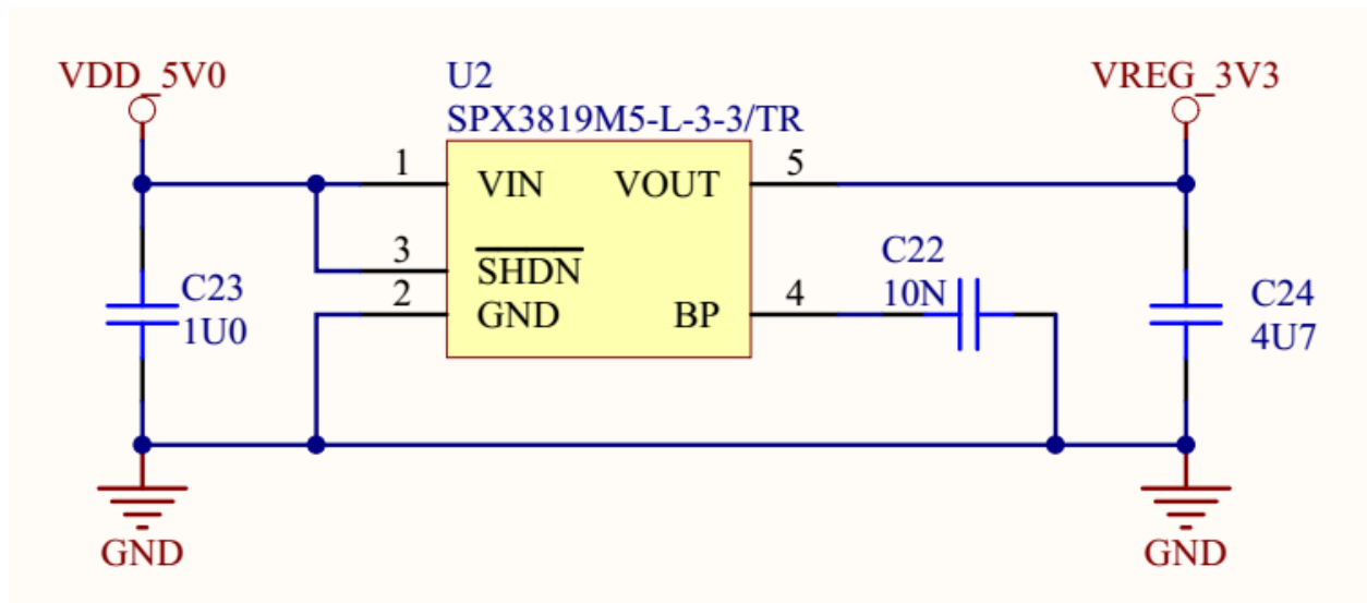
Figure 4-2 Power Supply
