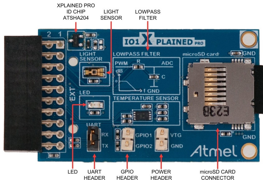
Figure 1-1 I/O1 Xplained Pro Extension Board
