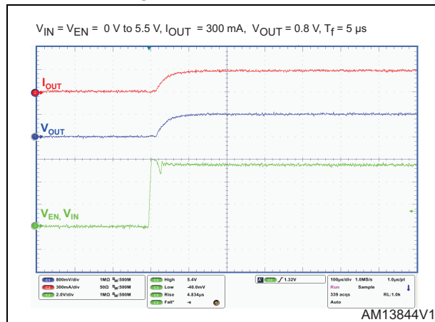
Figure 39. Turn-on time
