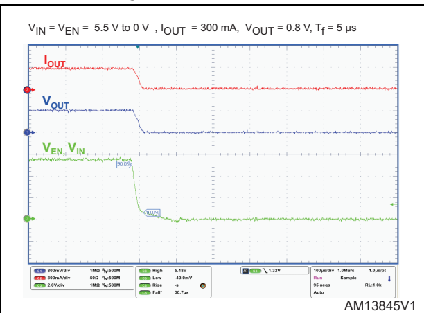
Figure 40. Turn-off time
