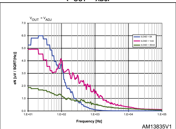
Figure 30. Noise spectrum vs. frequency ( V_{OUT} = V_{ADJ} )
