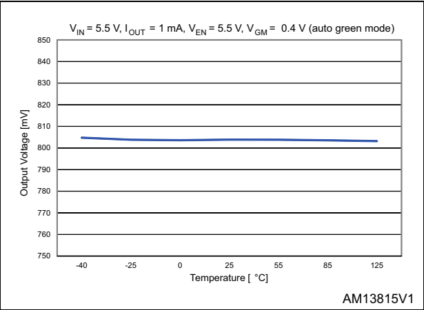
Figure 8. Output voltage vs. temperature ( V_{IN} = 5.5 V , I_{OUT} = 1 mA , auto green mode)
