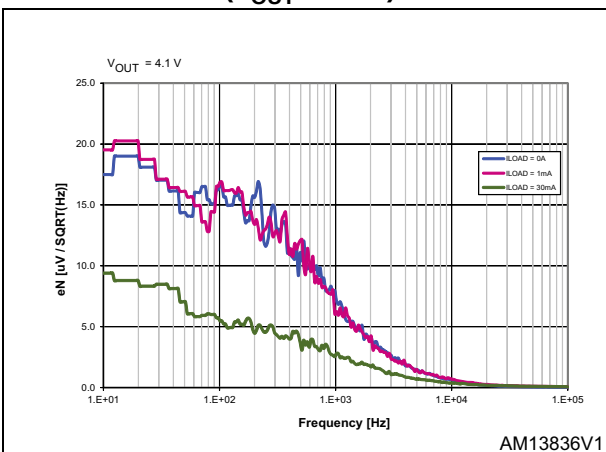
Figure 31. Noise spectrum vs. frequency ( V_{OUT} = 4.1 \text{ V} )
