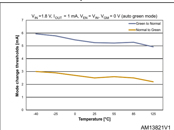
Figure 14. Mode change thresholds vs. temperature
