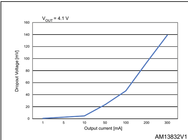
Figure 27. Dropout voltage vs. output current
