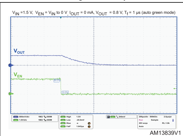
Figure 34. Turn-off by enable ( I_{OUT} = 0 mA, auto green mode)
