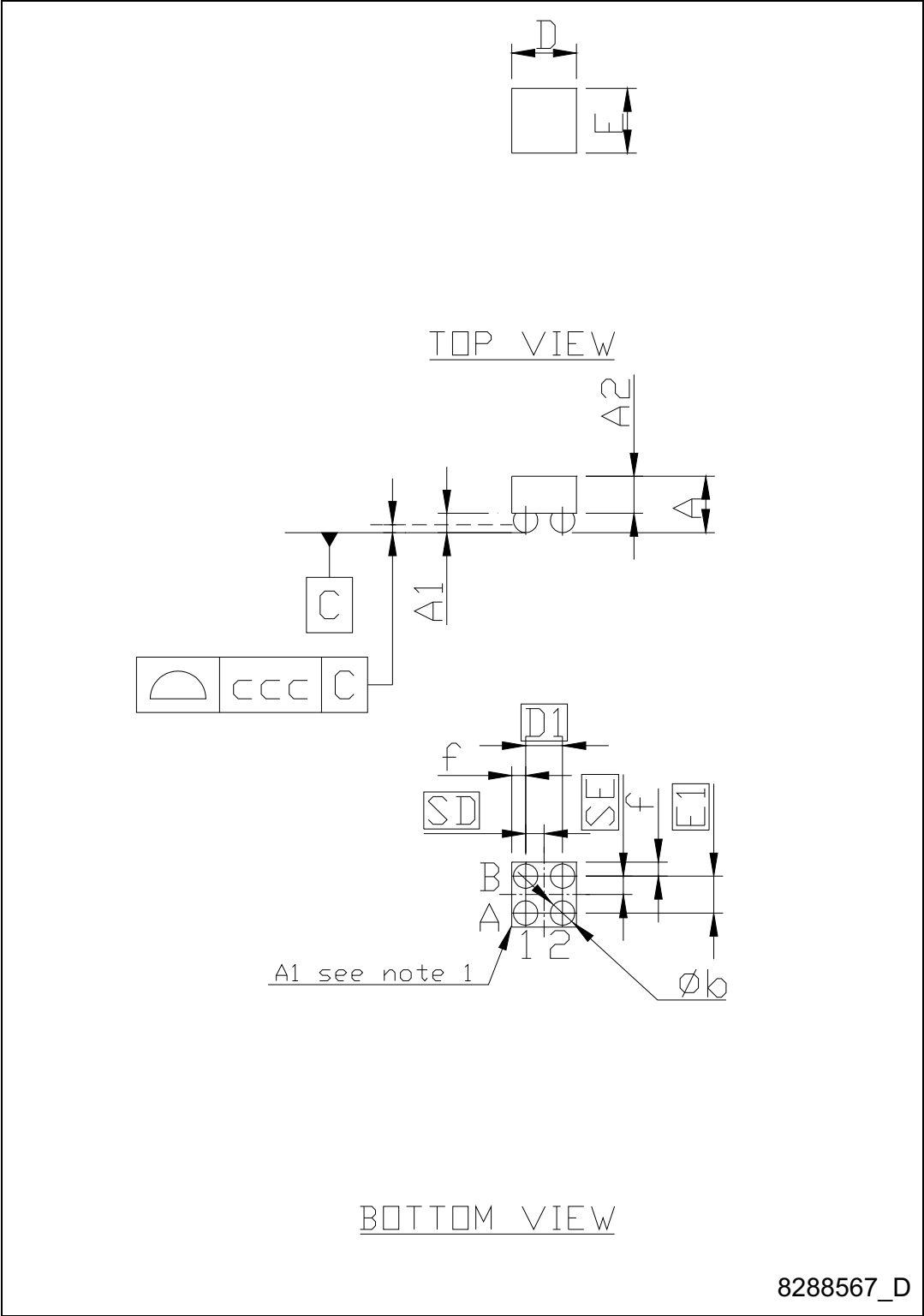
Figure 47. Flip-chip 4 drawings
