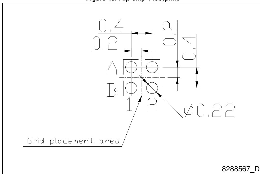
Figure 48. Flip-chip 4 footprint
