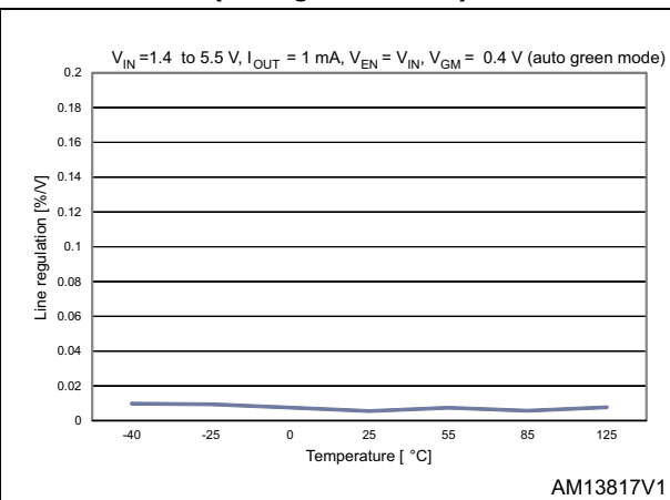
Figure 10. Line regulation vs. temperature (auto green mode)
