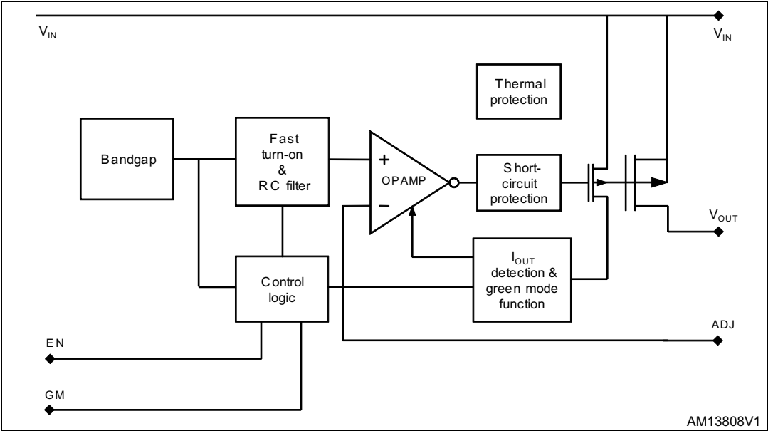
Figure 1. Block diagram (adjustable version)
