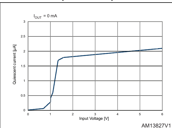
Figure 20. Quiescent current vs. input voltage (normal mode)
